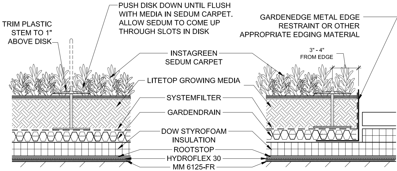
DISK ANCHOR SECUREMENT
