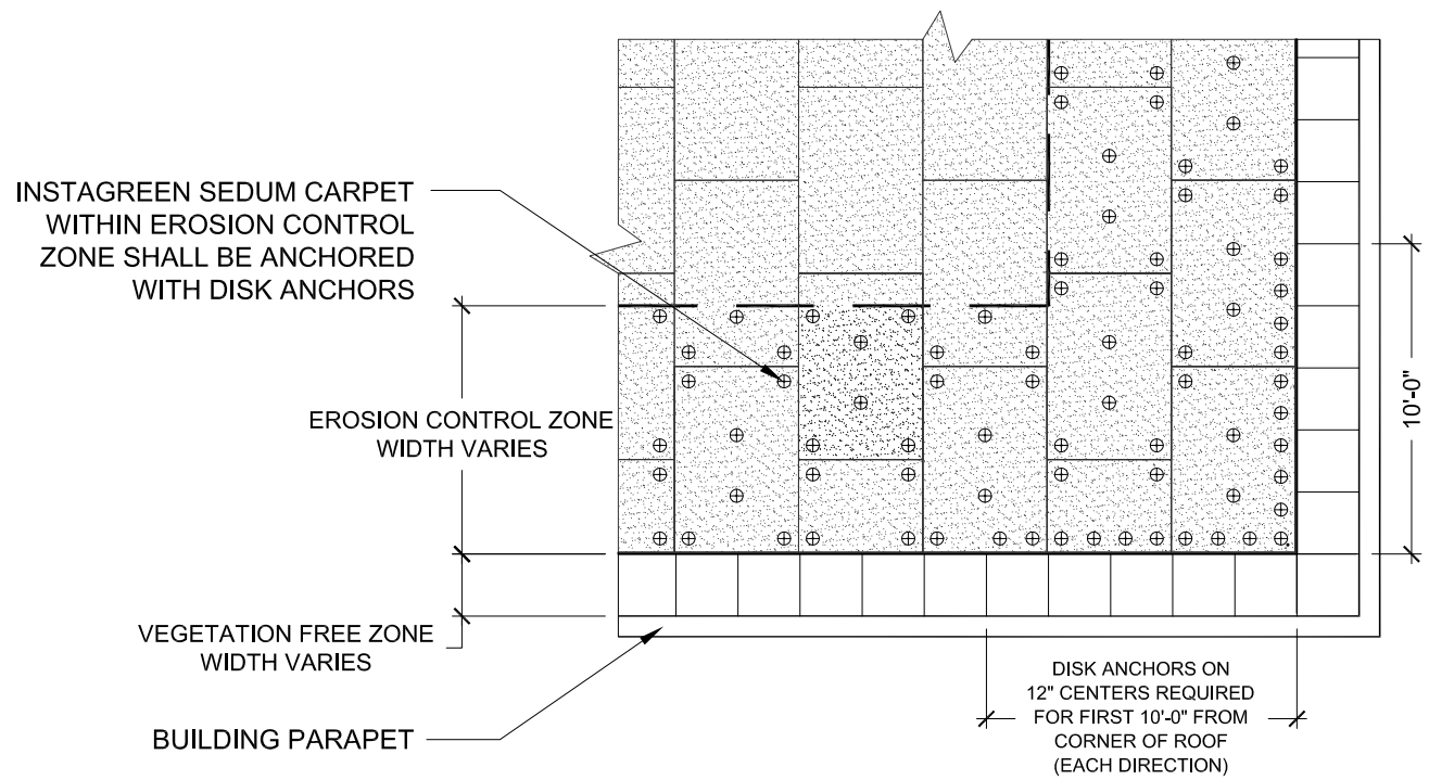
LAYOUT AND ANCHORING
